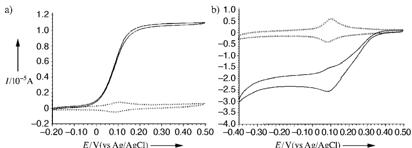
Figure 4. a) Cyclic voltammograms of I with co-electrodeposited GOX in PBS buffer: no glucose ( \circ ), 20 mM glucose (—). b) Cyclic voltammograms of I with co-electrodeposited SBP in PBS buffer: no \text{H}_2\text{O}_2 ( \circ ), 1.0 mM \text{H}_2\text{O}_2 (—). 3-mm vitreous carbon electrodes, pH 7.1, scan rate 5 \text{ mV s}^{-1} .
