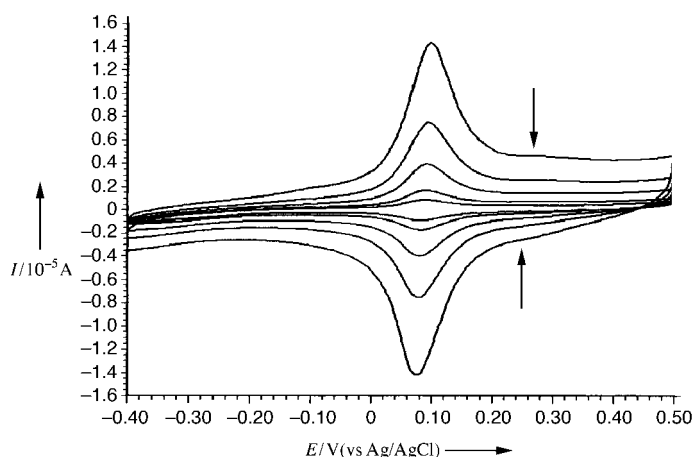
Figure 2. Cyclic voltammograms of the fully annealed film of I on vitreous carbon. pH 7.1, PBS buffer. Scan rates from the innermost to the outermost waves: 10, 20, 50, 100, and 200 \text{mV s}^{-1} . The approximate positions of the peaks of the waves of the crosslinking centers are marked with arrows.
